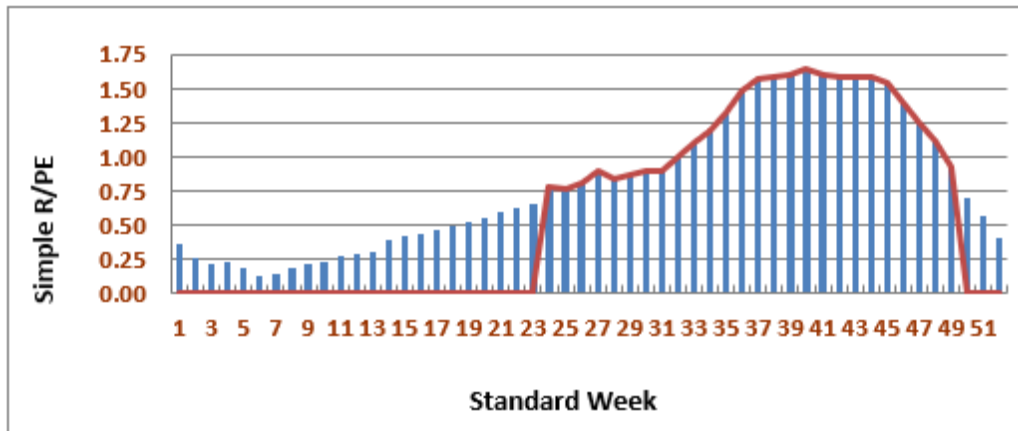
Fig 1: Karamadai region R/PE 14 week moving average 24 years (1992-2015)
