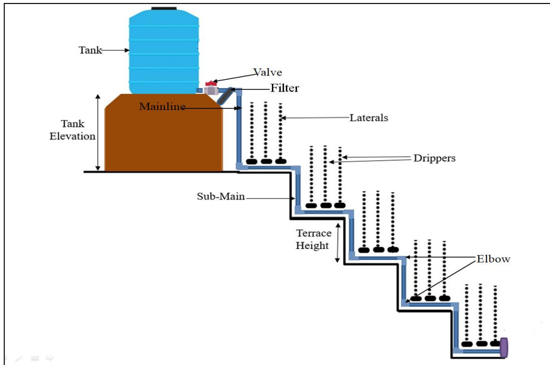
Figure 1: Basic set-up design for Gravity- Fed drip irrigation system for the terrace field (Source: Patle, 2020)
