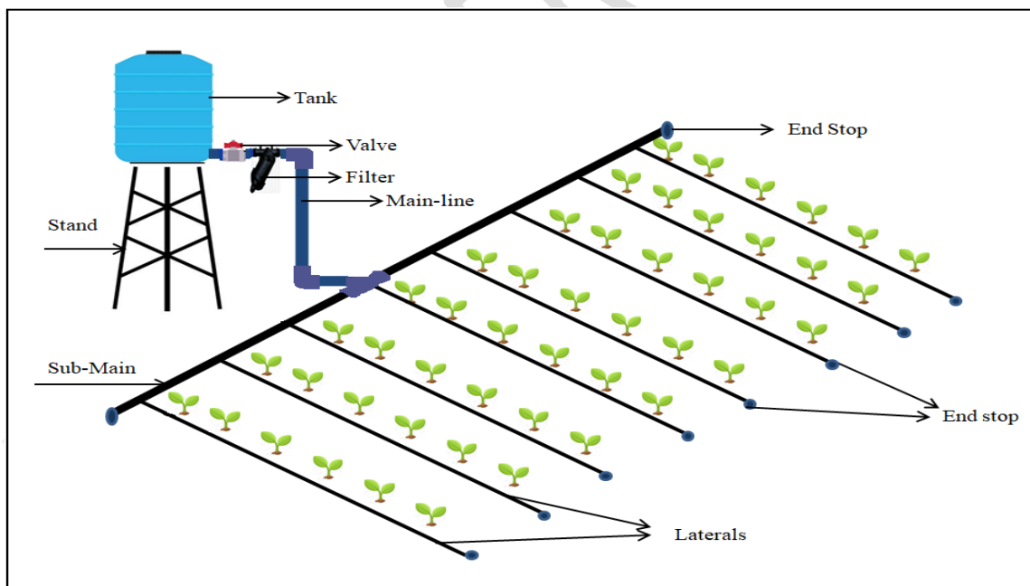
Figure 2. Drip irrigation layout for the level field area.
