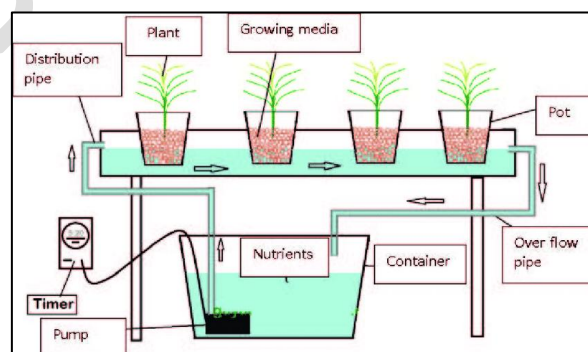
Fig.2 Nutrient Film Technique
