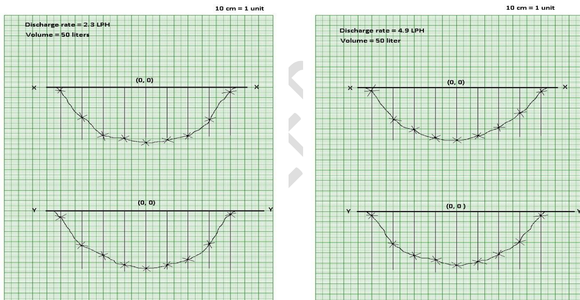
Figure.1 The depth of penetration of water at different points from the centre of wetting for both the x-sections
