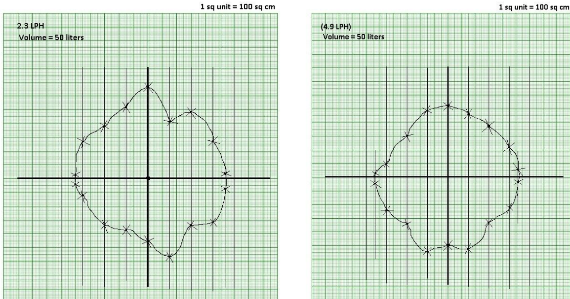
Figure.2 Width of wetting of water from the centre
