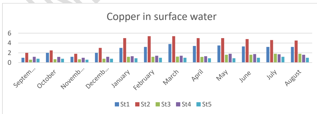
Fig 3: Copper (Cu) in surface water
