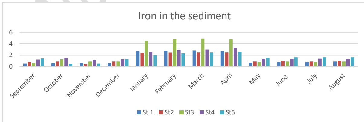
Fig 9: Iron (Fe) in Sediment
