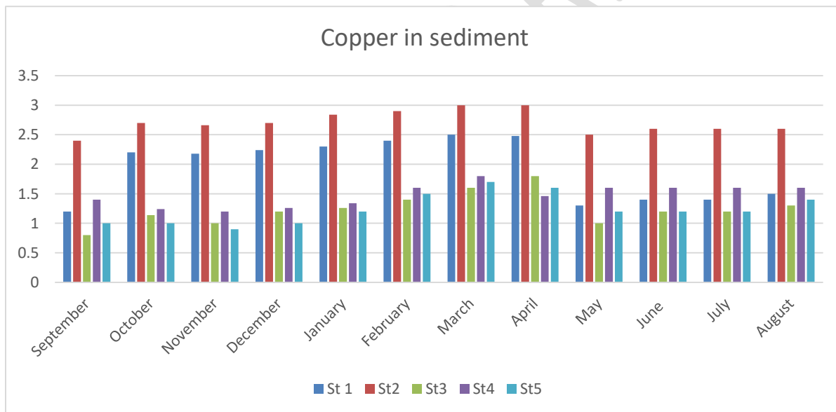
Fig 7: Copper in sediment
