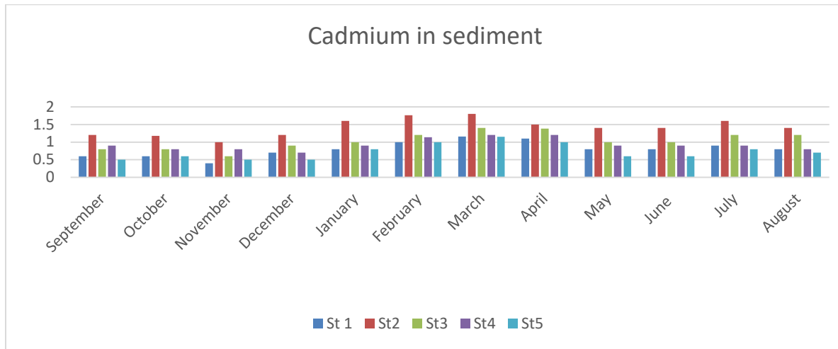
Fig 6: Cadmium (Cd) in Sediment
