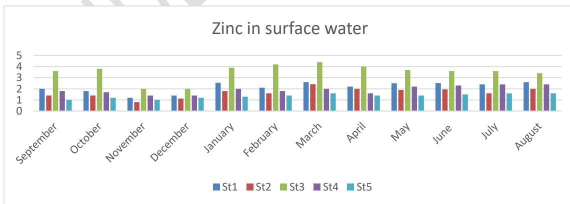
Fig 4: Zinc in Surface water.
