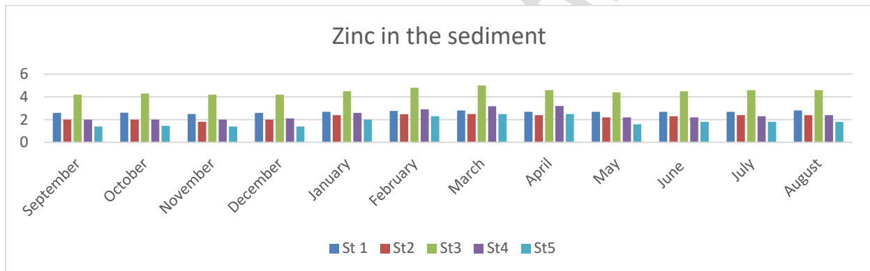
Fig 8: Zinc in Sediment
