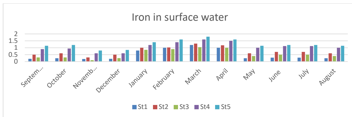
Fig 5: Iron (Fe) in Surface water.
