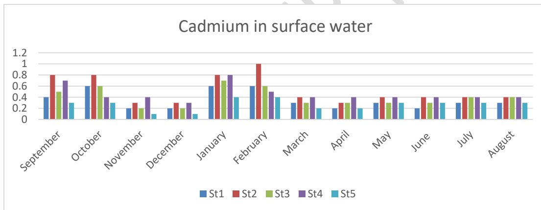
Fig 2: Cadmium (Cd) in surface water
