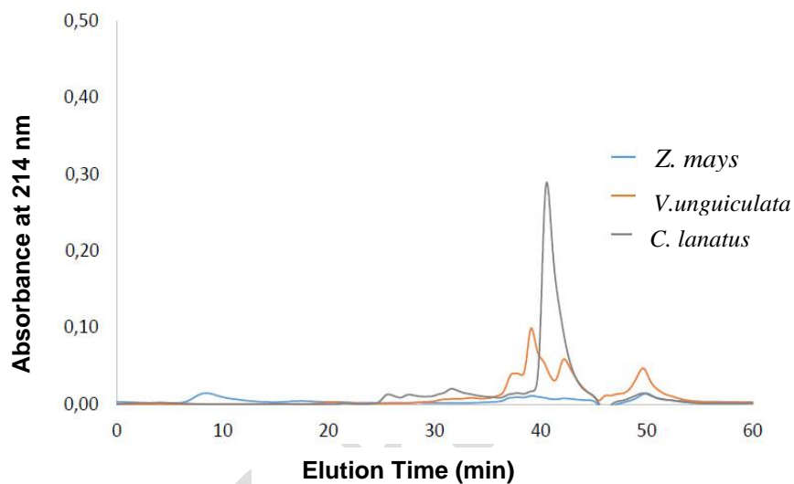
Figure 3. HPLC profiles of aqueous extracts 204-35000 Da
