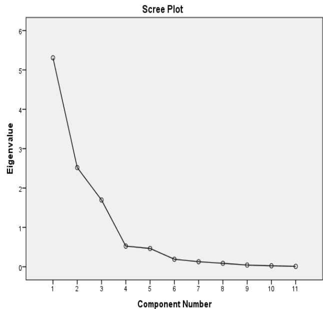
Fig. 2: Scree Plot showing variation of eigen values
