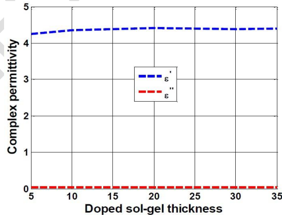
Fig. 5. Recap on the complex permittivity of sol-gel layers of different concentrations and thicknesses
