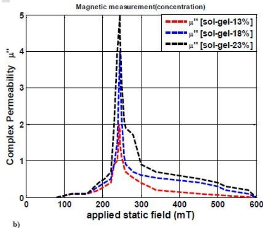
Figure 7. Variation of permeability \mu'' as a function of applied field for doped sol-gel
