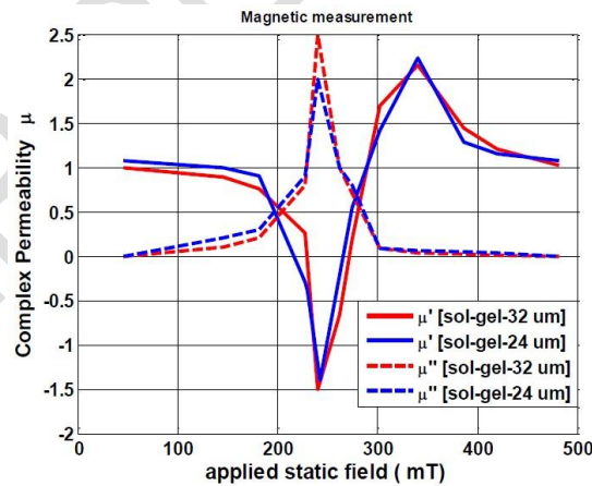
Fig. 4. Variation of complex permeability as a function of a doped sol-gel applied field with same concentration and two thicknesses
