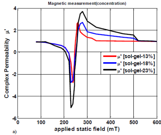
Fig. 6. Variation of permeability \mu' as a function of applied field for a doped sol-gel
