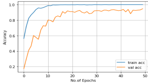
Fig 6 Train accuracy and validation accuracy
