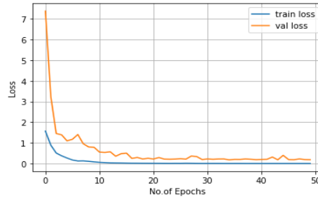
Fig 7 Train loss and validation loss
