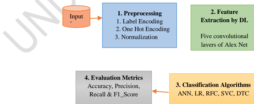
Fig.2 Framework for Disease Classification
