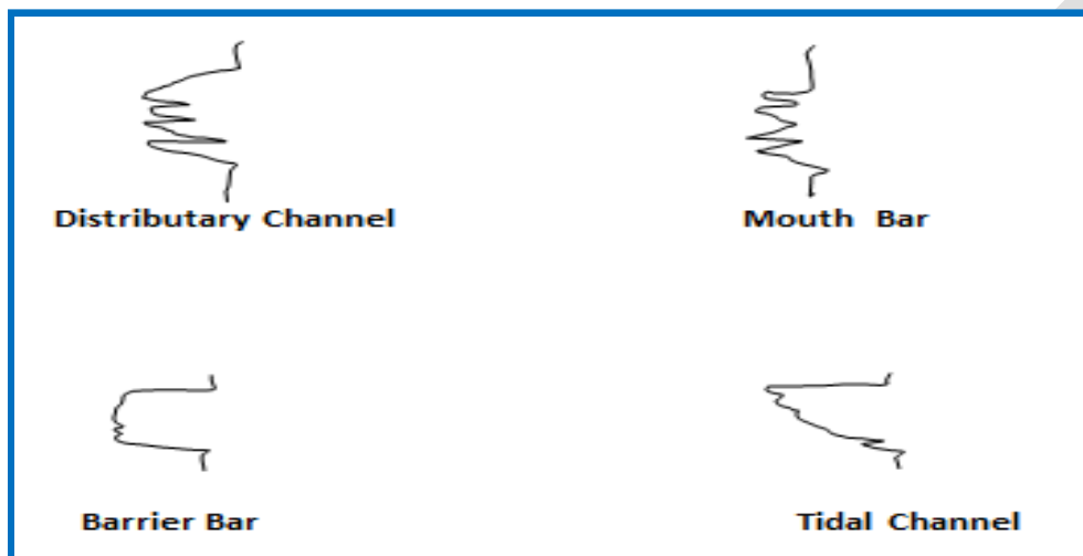
Fig. 9. Recognition of depositional environments using gamma logs from deltaic reservoirs (After, Scumberger, 1985).
