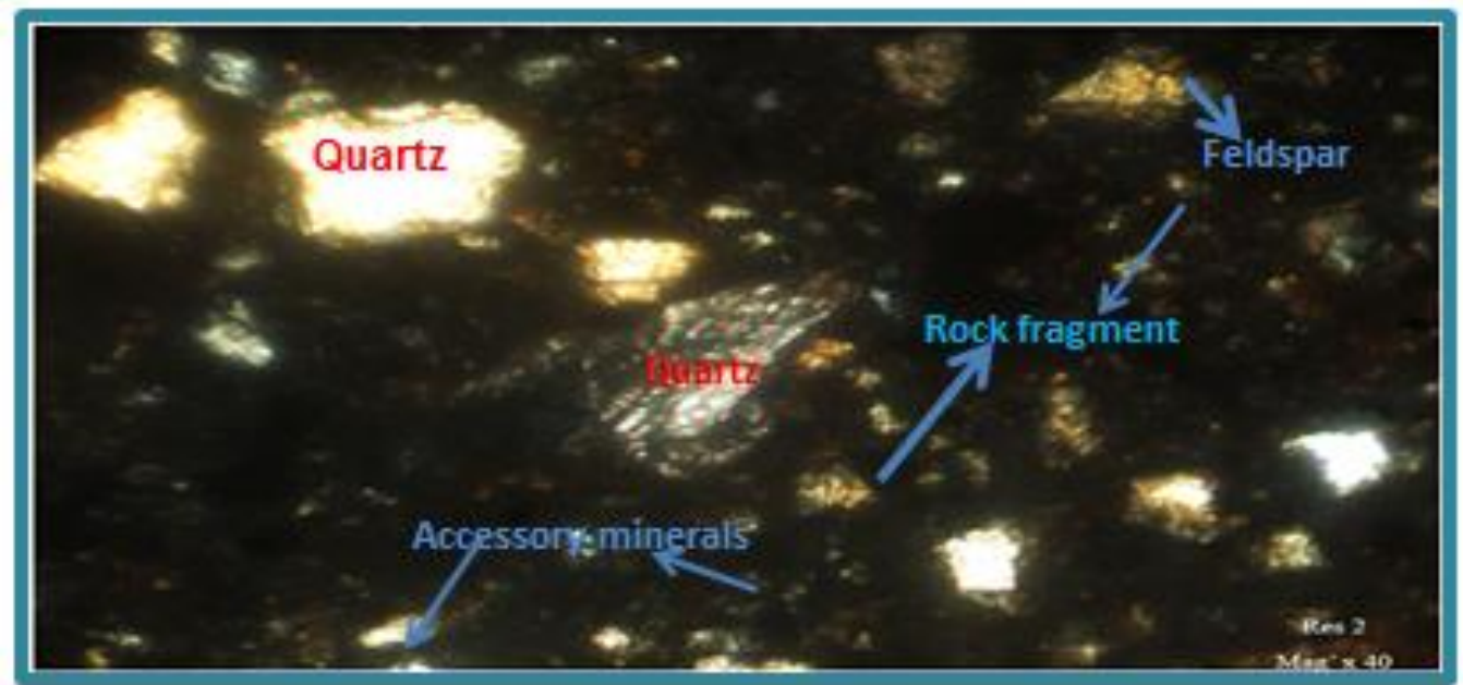
Fig. 5. Photomicrograph of the reservoir sands in the distributary channel depositional environment.
