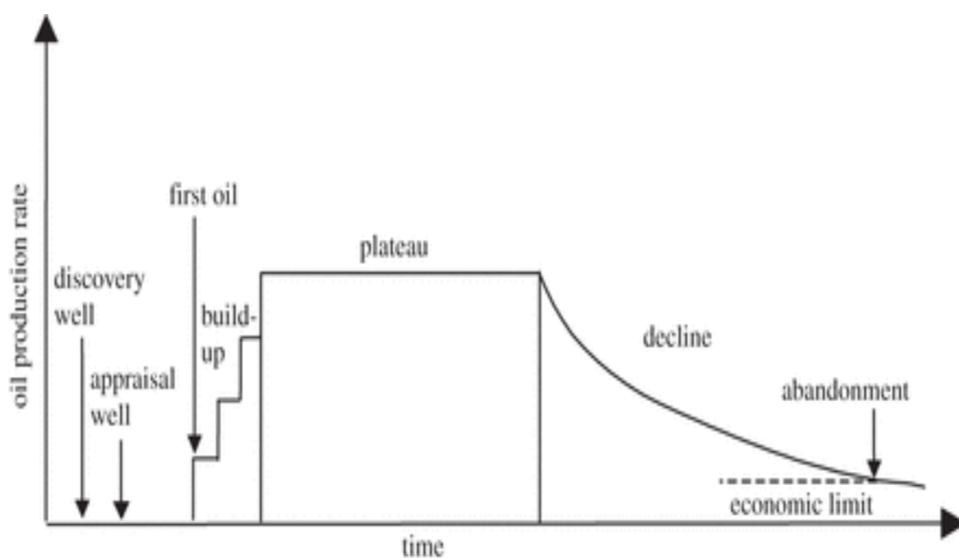
Image 1. Idealized production behaviour of an oilfield. Source: Höök et al. [2].
