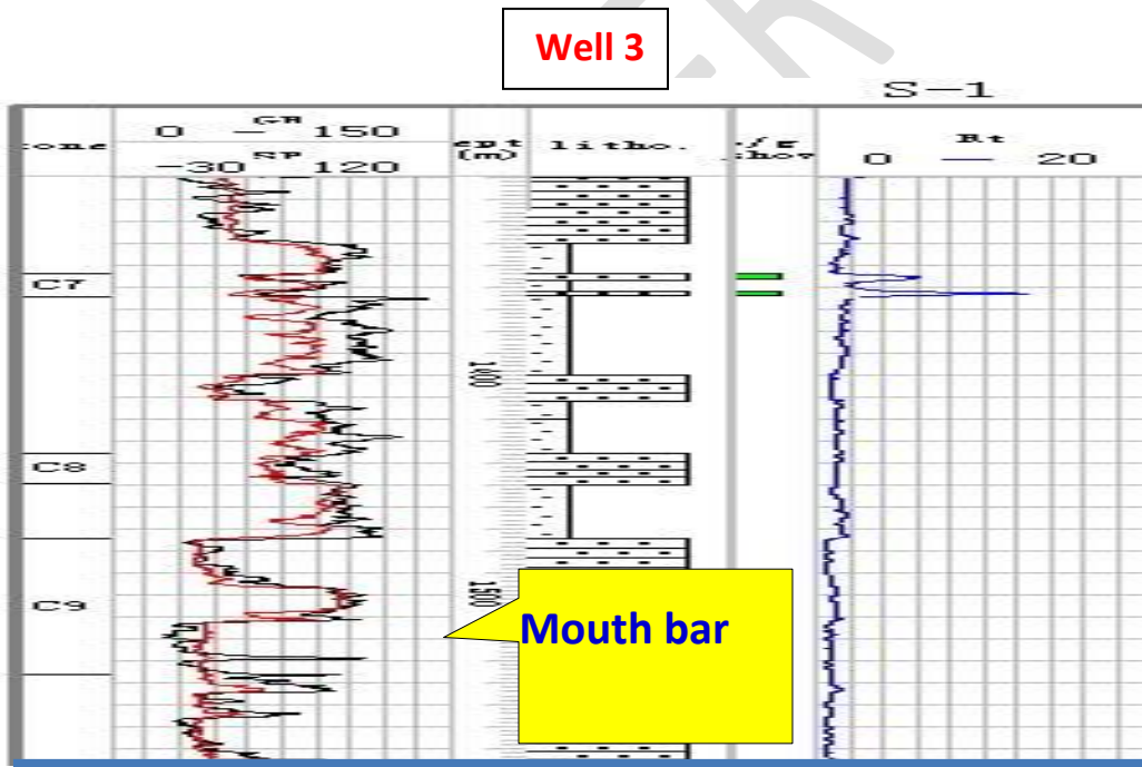
Fig. 4. Gamma ray log signature of Heri sand in well 3
