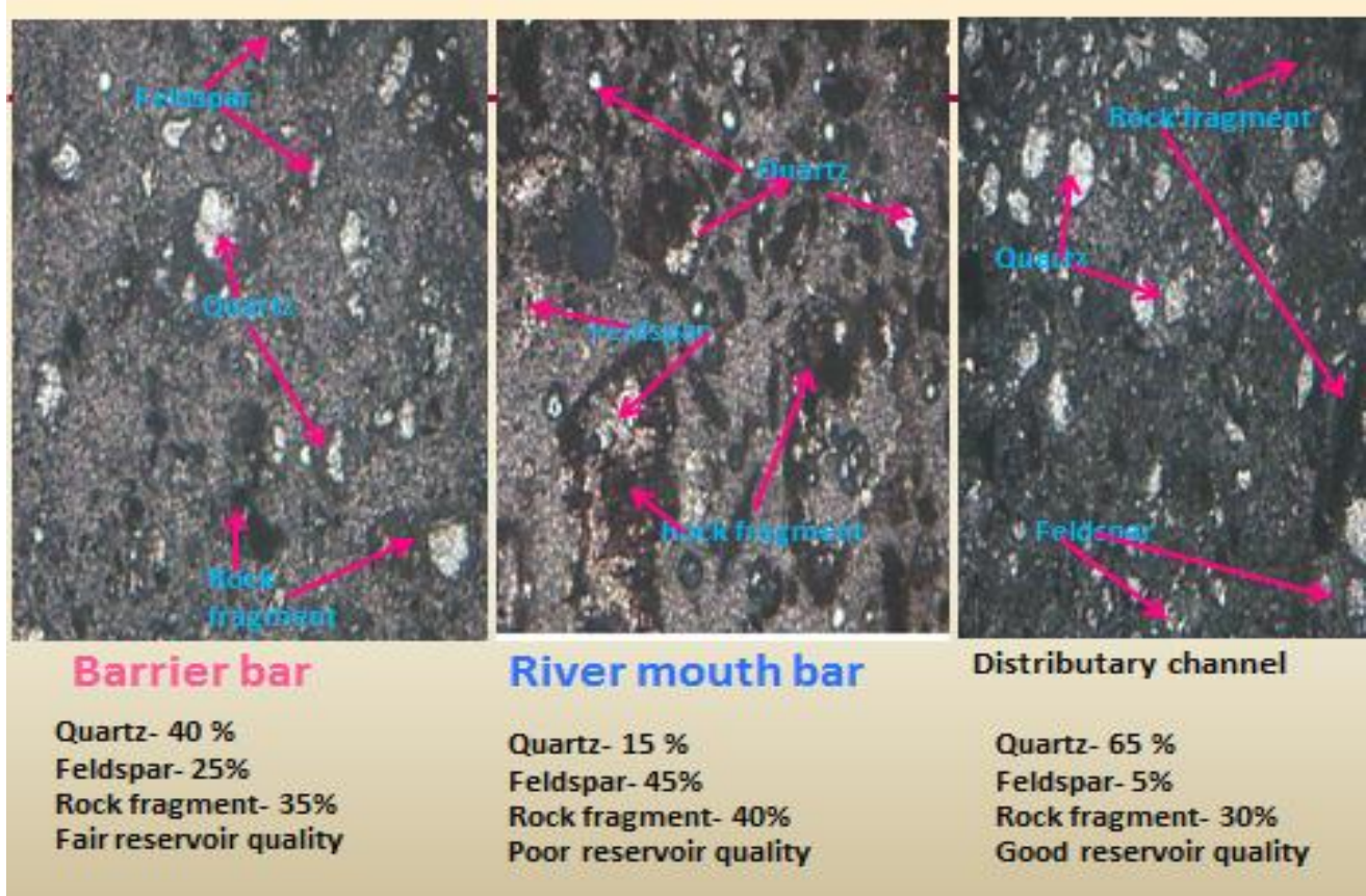
Fig 10. Photo micrograph of the representative units of depositional environments of the reservoir.
