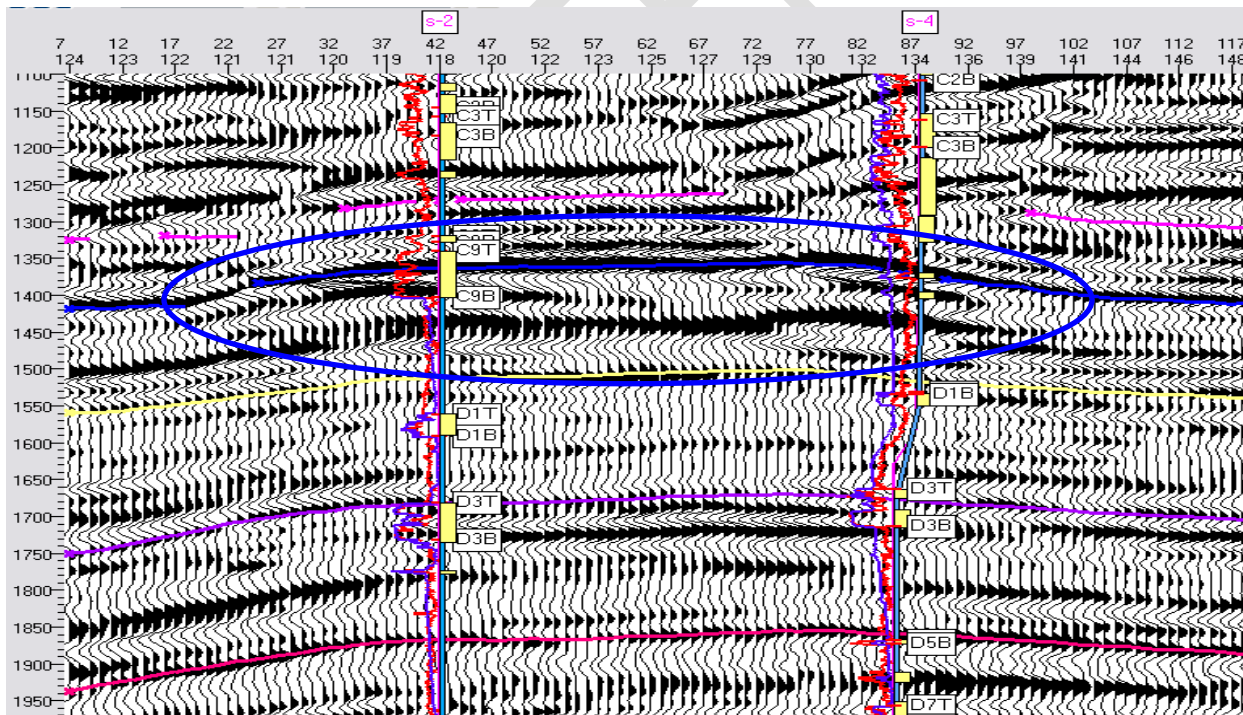
Fig. 2 Superimposition of seismic section on suite of well logs penetrated by the reservoir in the field
