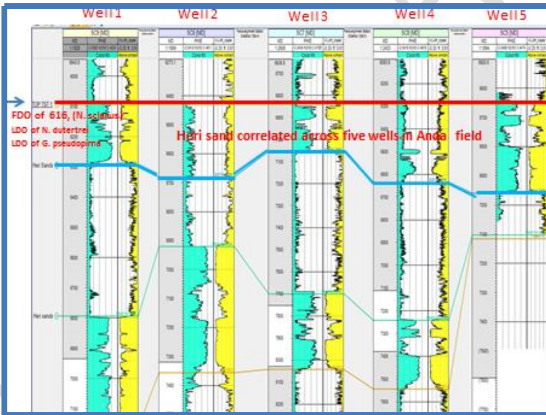
Fig. 8. Correlation of the reservoir across selected wells using well logs and biostratigraphic data.
