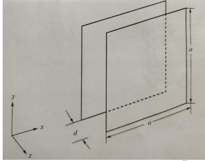
Fig.1 Schematic diagram of Casimir force
