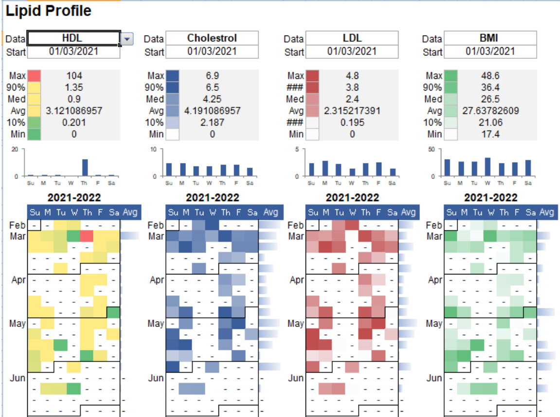
Figure 2. Calendar Plot for Lipid Profile
