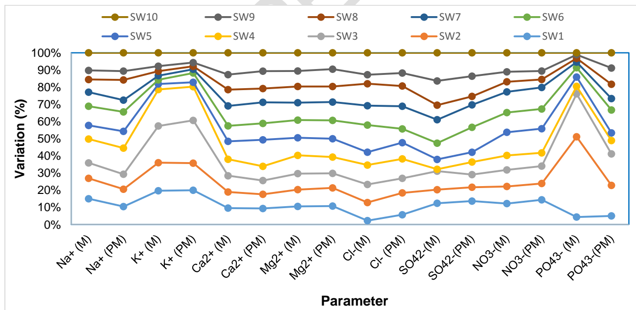
Figure 3. Seasonal variation of chemical attributes of SW samples in monsoon and post-monsoon season
