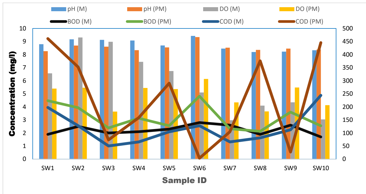
Figure 2. Seasonal variation of physical attributes in SW samples
