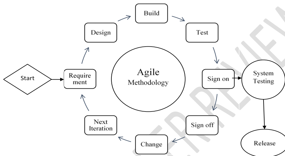
Figure 1: Agile Model
