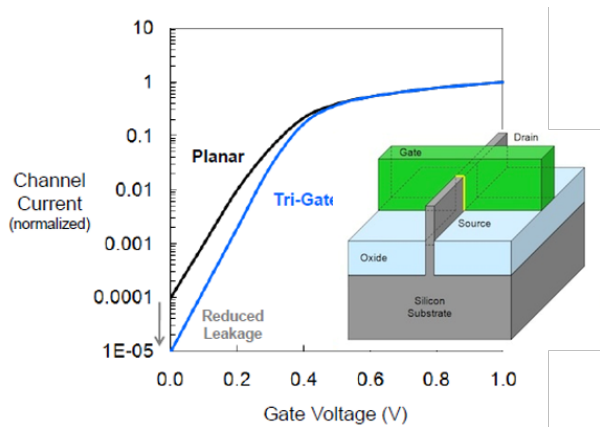
Fig. 8. Trigate transistors
