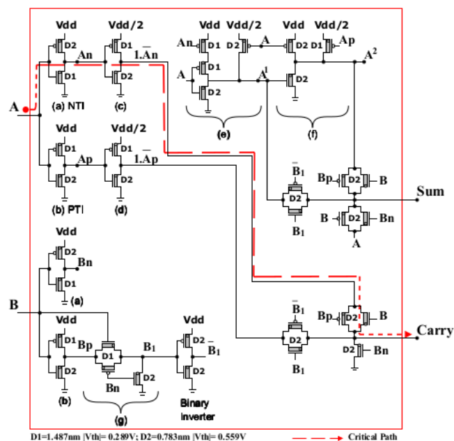
Fig. 12. A ternary Half Adder
