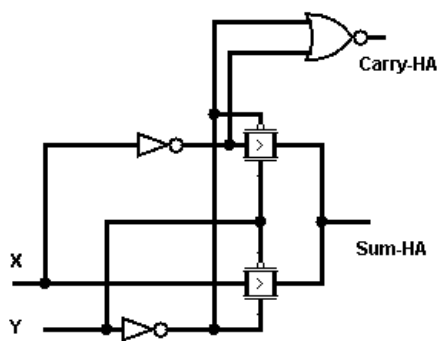
Fig. 13. Binary Half Adder (MUX technique)
