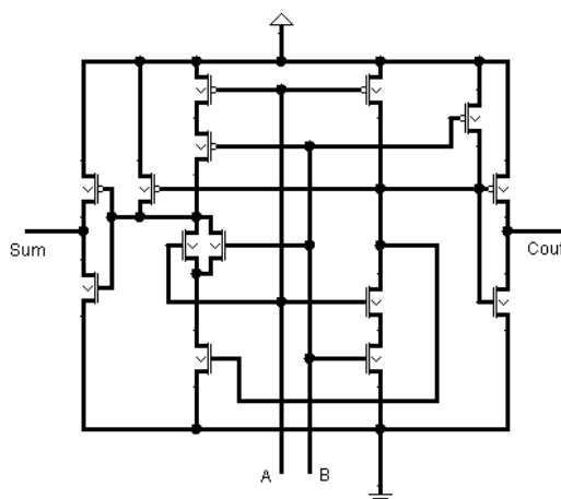
Fig. 14. 14 T binary Half Adder)
