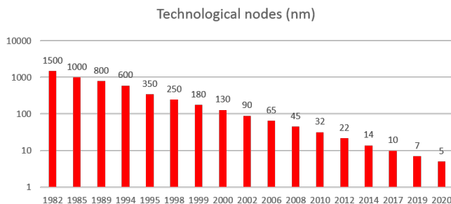
Fig. 9. CMOS technological nodes
