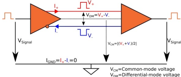
Fig. 6. Differential signaling
