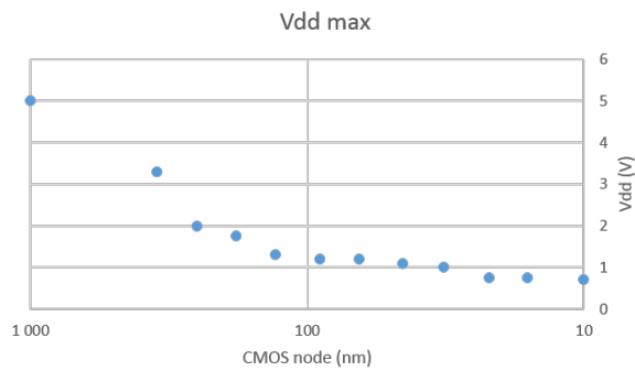
Fig. 7. V dd scaling since 1000-nm node
