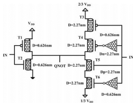
Fig. 3. A 4-valued CNTFET inverter [8]
