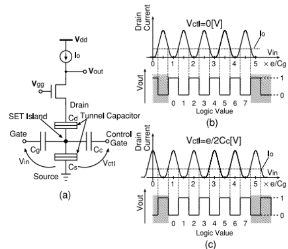
Fig. 11. SET periodical literal circuit (a)Schematic, (b) and (c) transfer characteristics for two V_{ctl} values
