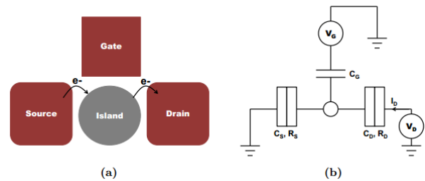
Fig. 10. (a)Schematic of SET ; (b) Schematic of equivalent circuit
