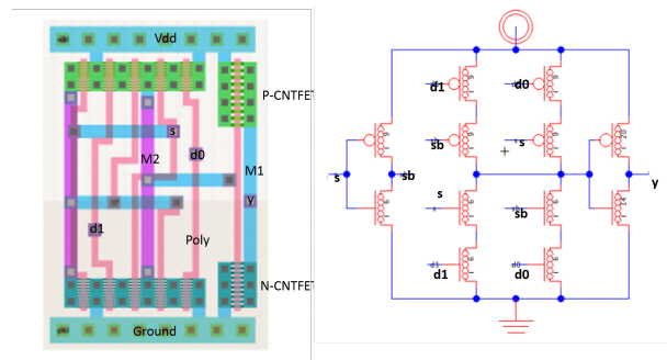
Fig. 4. 2:1 CNTFET multiplexer. Layout (left) and circuit (right)
