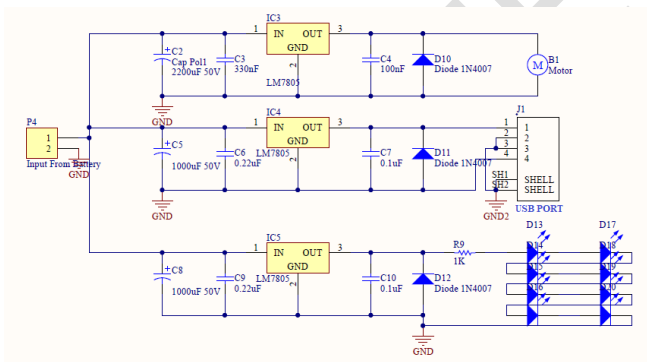
Fig. 4. Schematics of discharging circuit
