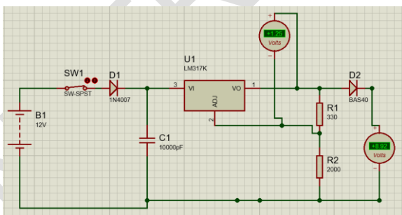
Fig. 5. Simulation schematic of charging circuit
