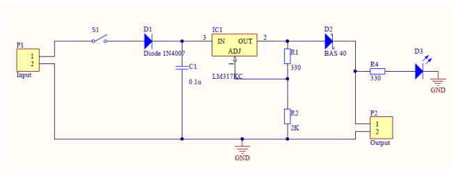
Fig. 3. Schematics of charging circuit
