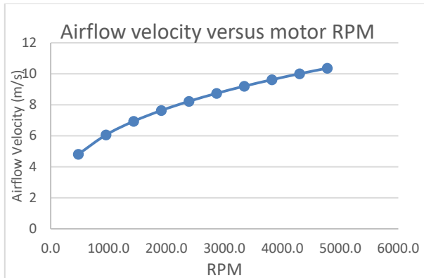
Fig. 9. Relation of airflow velocity and motor RPM
