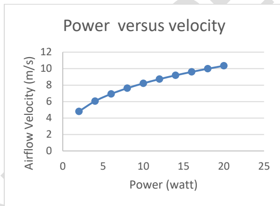
Fig. 8. Relation of power and airflow velocity
