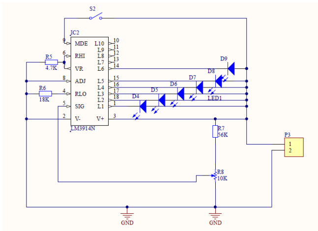
Fig. 2. Battery voltage level indicator circuit
