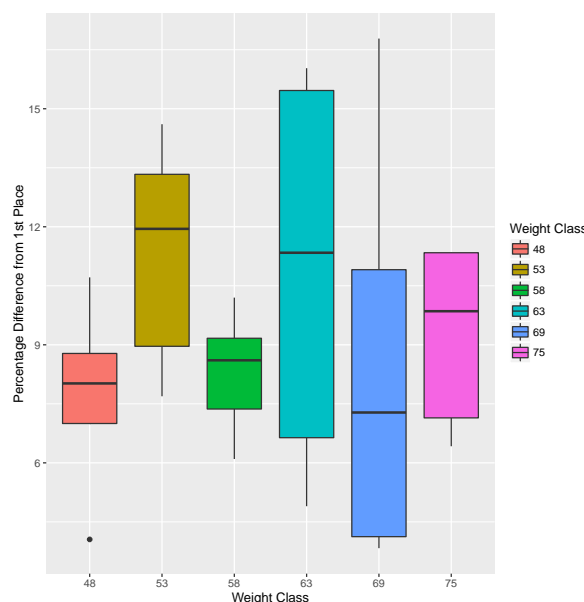
Figure 4: Boxplot of the percent difference of 5th place lifters from Gold medalist for female weight classes
