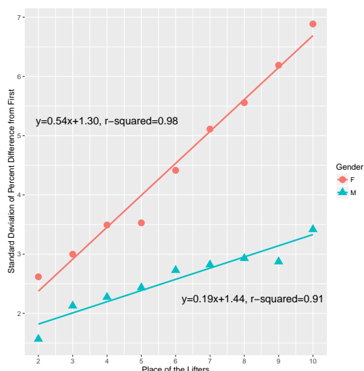
Figure 2: Standard deviation of the percent difference from first as the place a lifter attains changes
