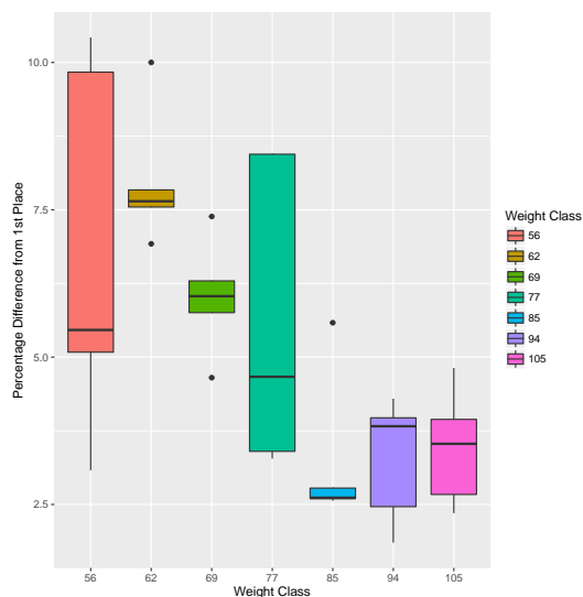
Figure 3: Percent difference of 5th place lifters from Gold
