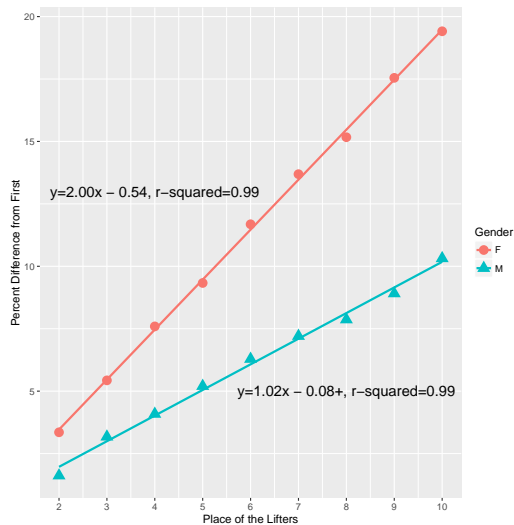
Figure 1: Scatterplot of mean percent difference from a first place lifter and place a lifter attains
