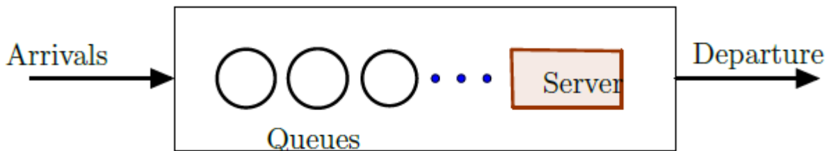
Figure 2: Single-Server, Single-Phase System
