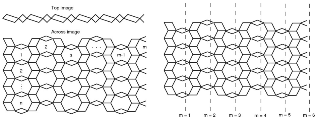
Figure 3: The molecular graph of TiO_2[n, m] nanotube.
