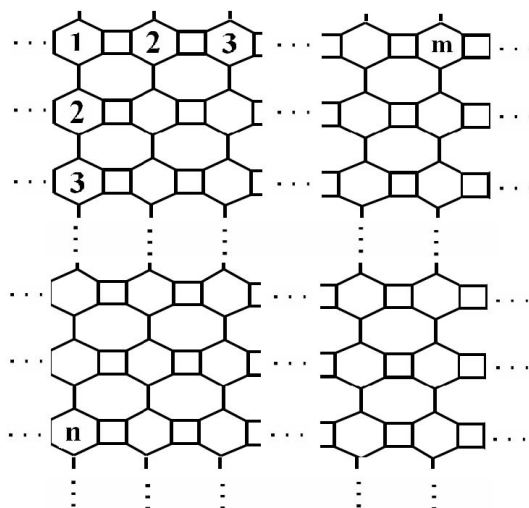
Figure 2: The molecular graph of VPHY[m, n] nanotorus.
