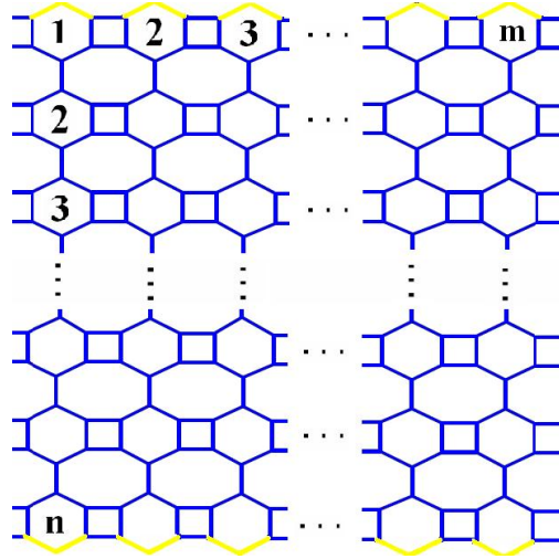
Figure 1: The molecular graph of VPHX[m, n] nanotube.
