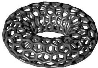
Figure 4: molecular graph of a nanotorus
