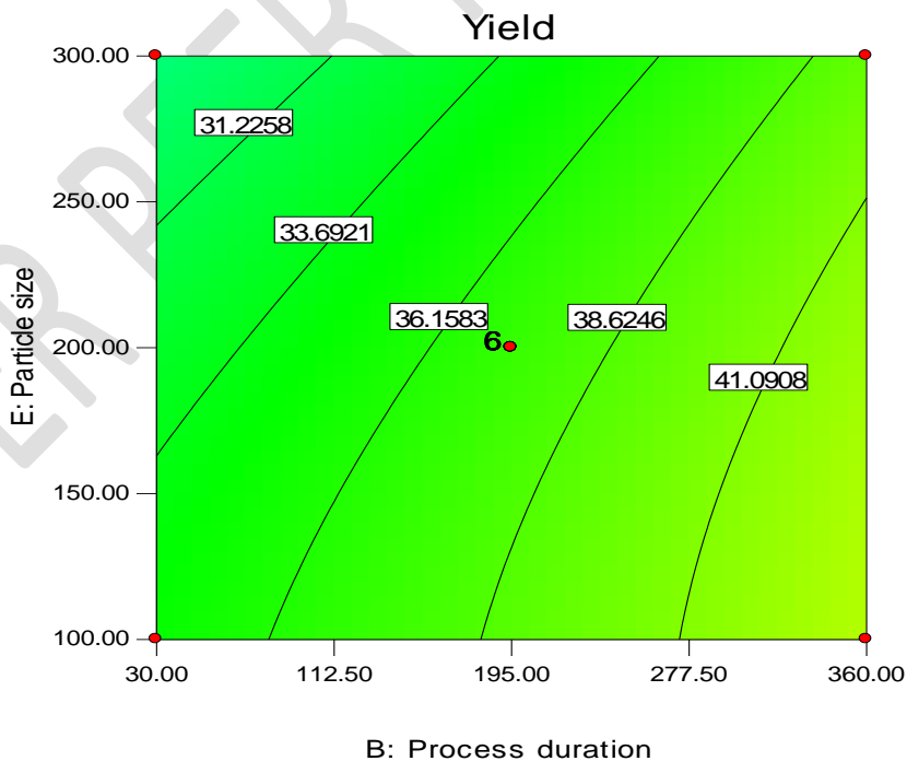
Figure 12: The contour plots for particle size against process duration and yield of AAC
