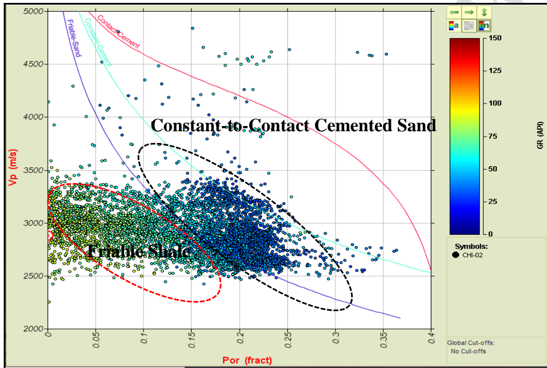
Fig. 3a: Cross plots of Velocity against Porosity Color-coded With gamma ray
