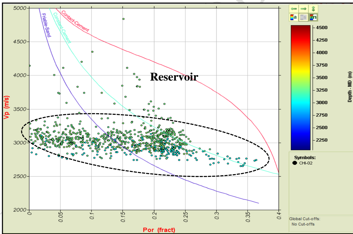
Fig. 4a: Cross-plots of Velocity against Porosity Color-coded at reservoir interval with Depth for CHI-02 Well
