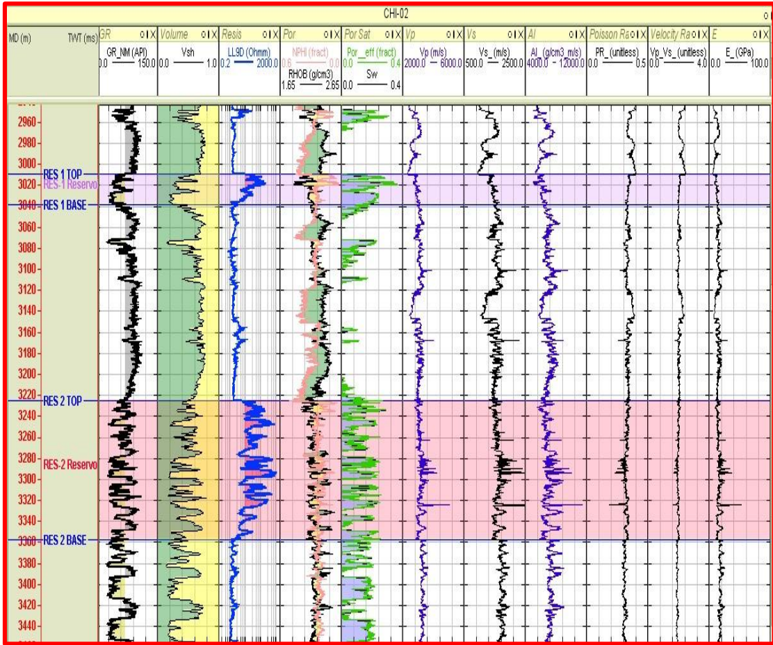
Fig. 5a: Log Plots of Elastic and Reservoir Parameters Generated for CHI-02 Well
