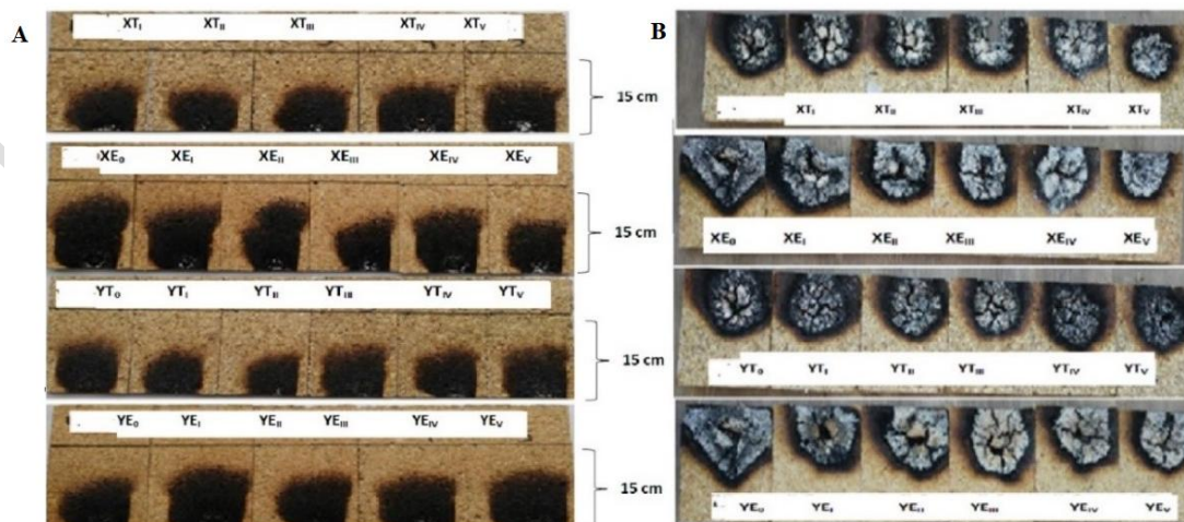
Figure 1. The fire behaviors on the experimental panels which exposed to a single flame source (A: Flame spread according to TS EN-ISO 11925-2, B: Combustion behaviors of panels).
