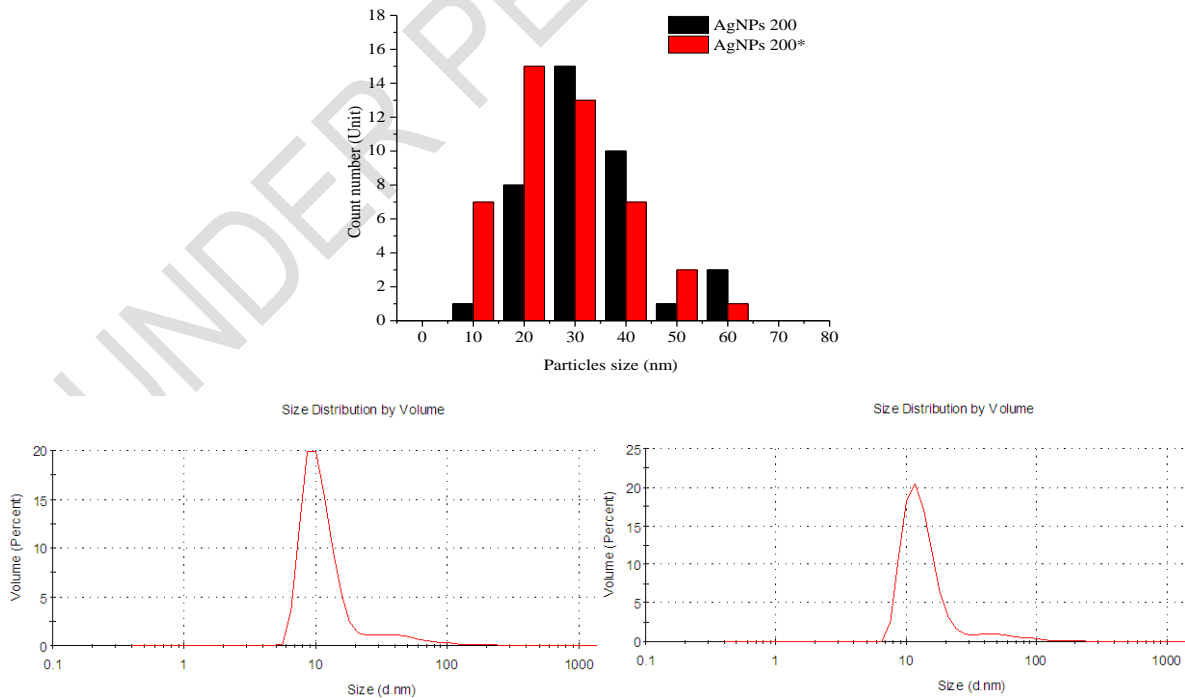
Fig. 6 Particle size distribution (a) size distribution by volume of AgNPs 200* (b) AgNPs 200 (c)
