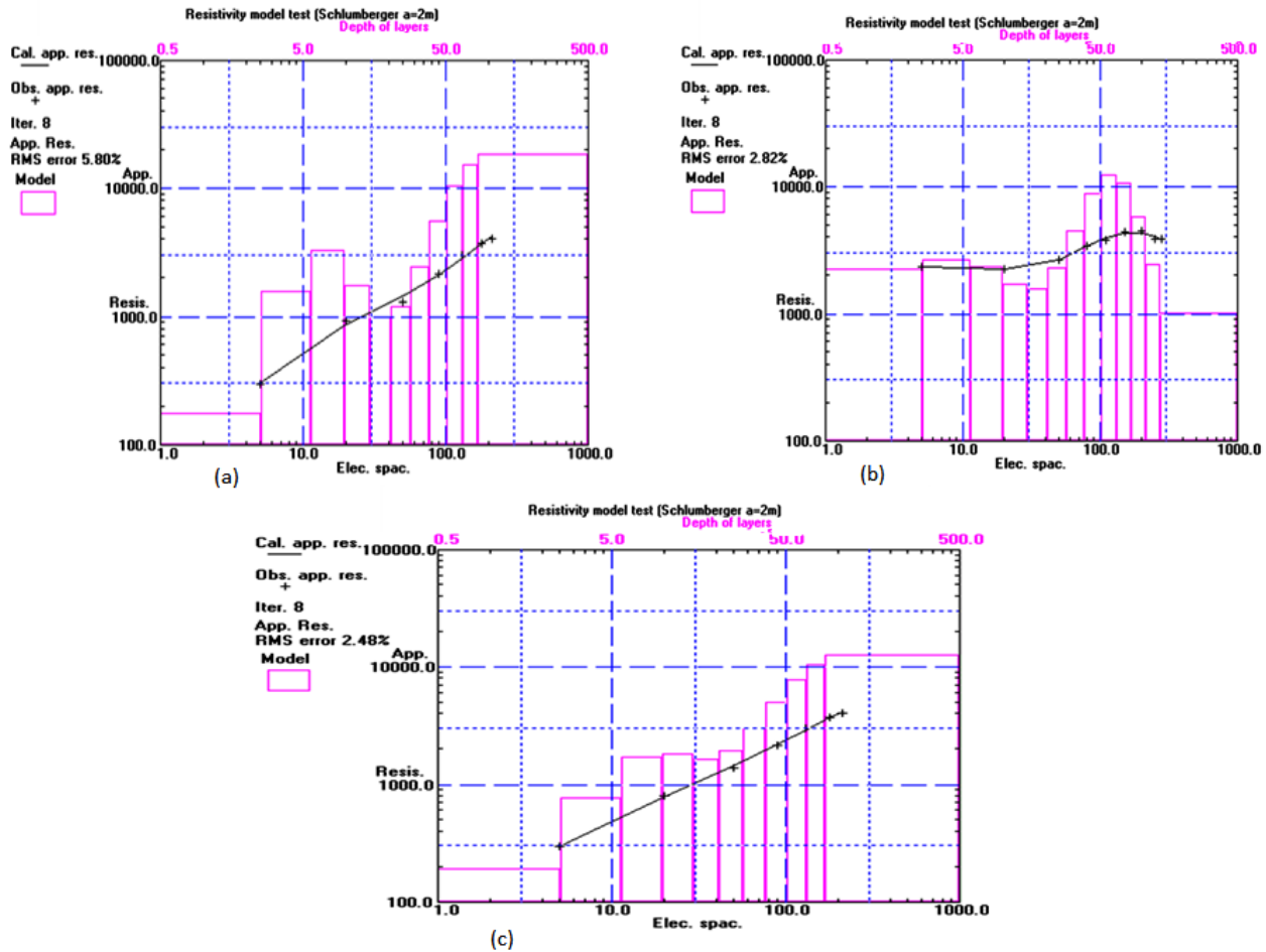
Fig. 6: (a) Inverted model layer for VES 5 taken at Iguebe south (2) Inverted model layer for VES 6 taken at Ebelle (c) Inverted model layer for VES 7 taken at Ekpon in Edo State
