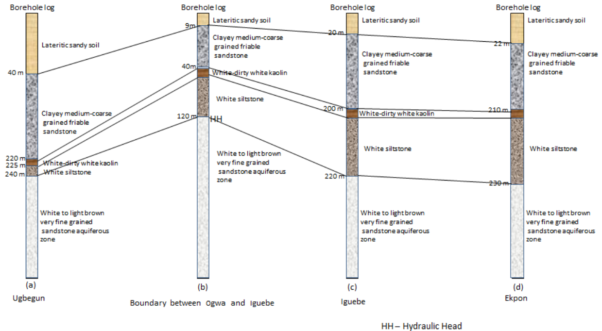
Fig.8:Litho-log of boreholes section of the study area(Source of borehole data: Rock Well Drilling Company)
