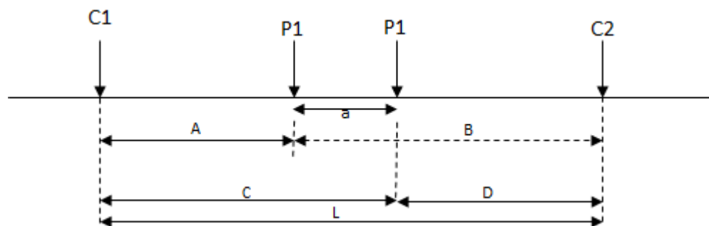
Fig. 4: Schlumberger array (After Lowrie, 1997)
