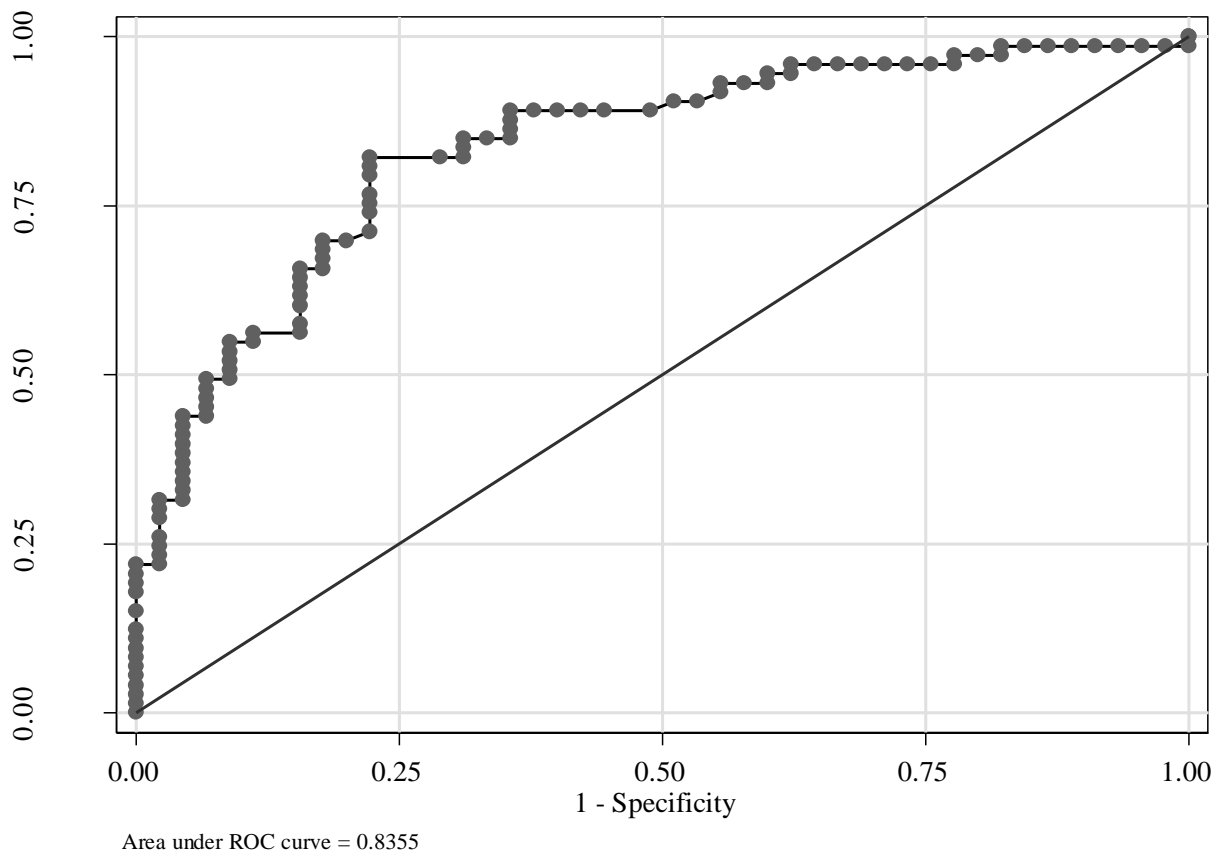
Figure 2:ROC Curve
