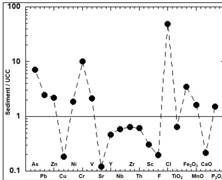
Figure 2. Comparison of trace and major element concentration in surface sediments of Conakry mangrove. All values were normalized to the UCC values of [13].
