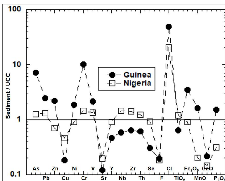
Figure 3. Comparison of trace and major element concentration in surface sediments of Guinea and Nigeria mangrove. All values were normalized to the UCC values of [13].
