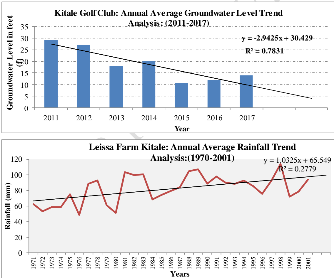
Figure 9: Kitale Golf Club Annual Average Groundwater levels and Leissa Farm Kitale Rainfall Bar Graphs
