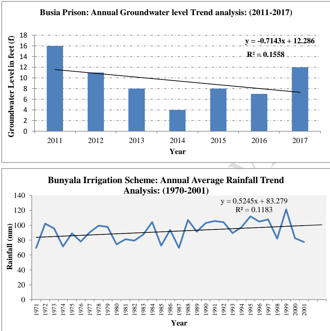
Figure 15: Busia Town Prison Annual Average Groundwater levels and Bunyala Irrigation Scheme Rainfall Bar Graphs
