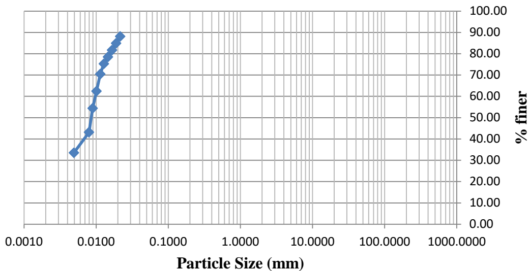
Figure 4: Particle size distribution of oturo sample
