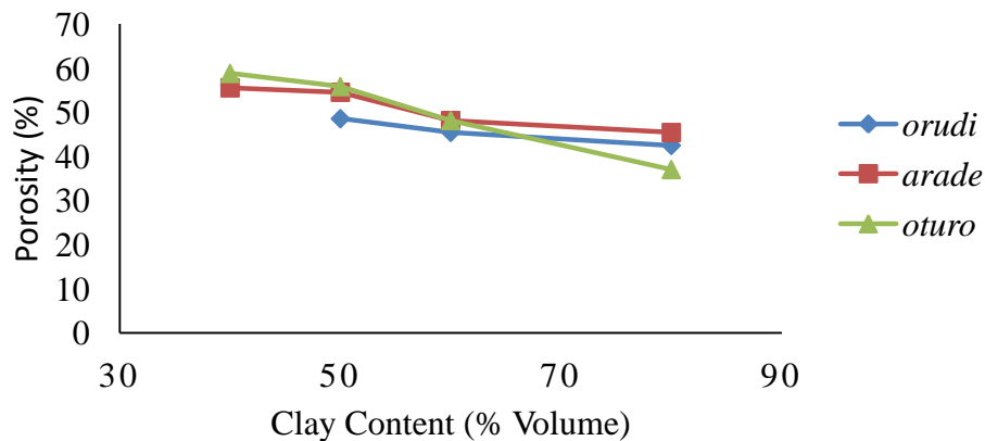
Figure 7: Effect of clay content on Porosity
