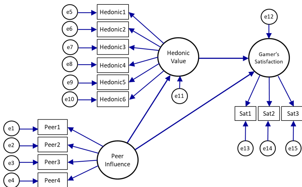
Fig. 2. Path diagram of the structured equation model
