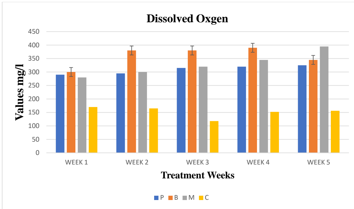
Fig 1: Dissolved Oxygen
