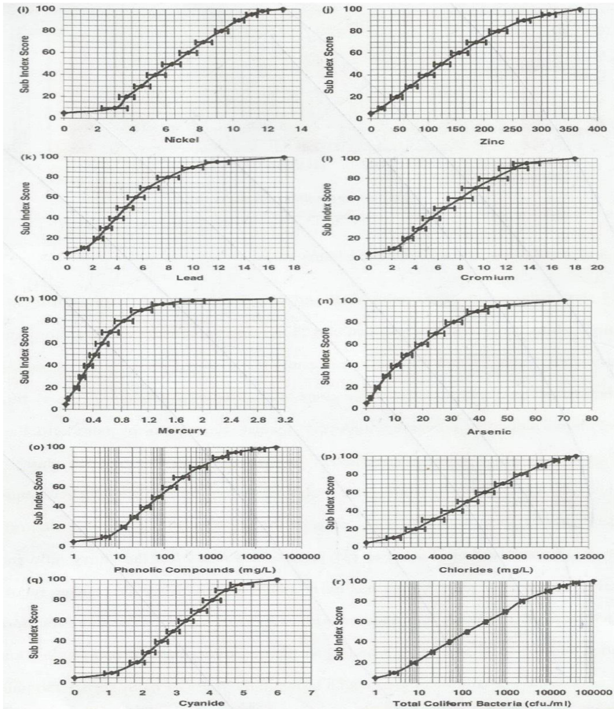
Figure 3.0: The average sub-index curves of pollutants [12]
