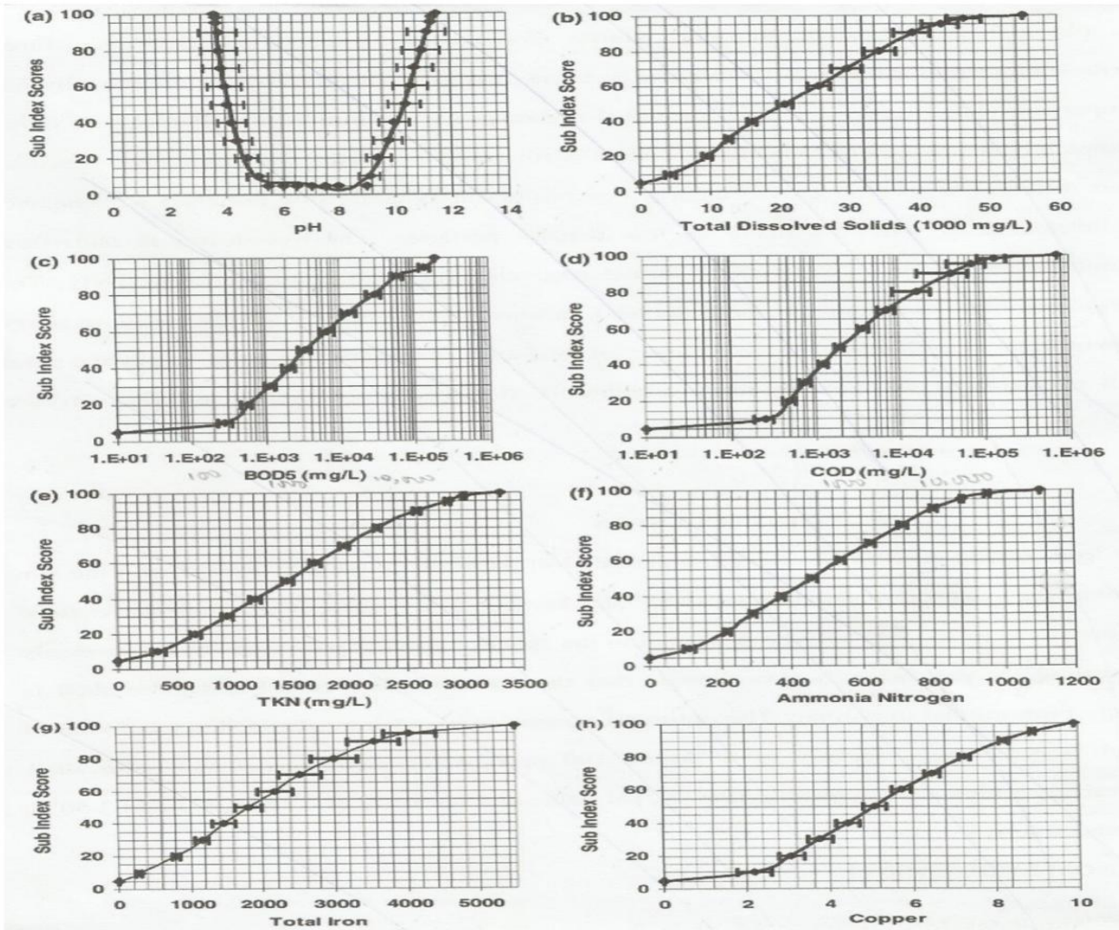
Figure 2.0: The average sub-index curves of pollutants [12]
