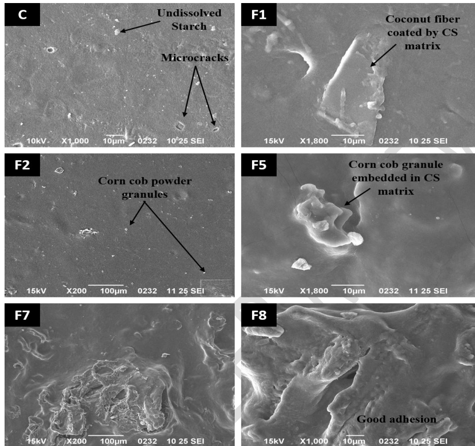
Fig. 7 – Scanning electron micrograph of biocomposite films. (C: control, F1, F2, F5, F7, F8: formulations)
