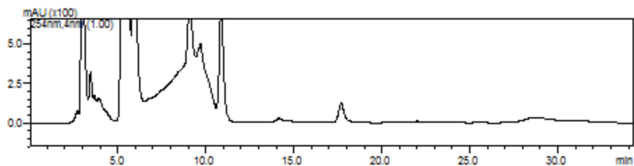
Figure 3. Sample chromatogram
