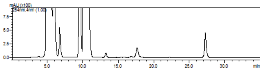
Figure 2. Standard chromatogram
