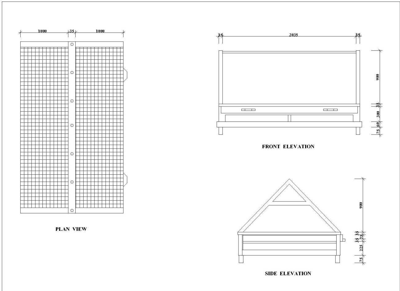
Figure 1: Orthographic view of a direct solar dryer.
