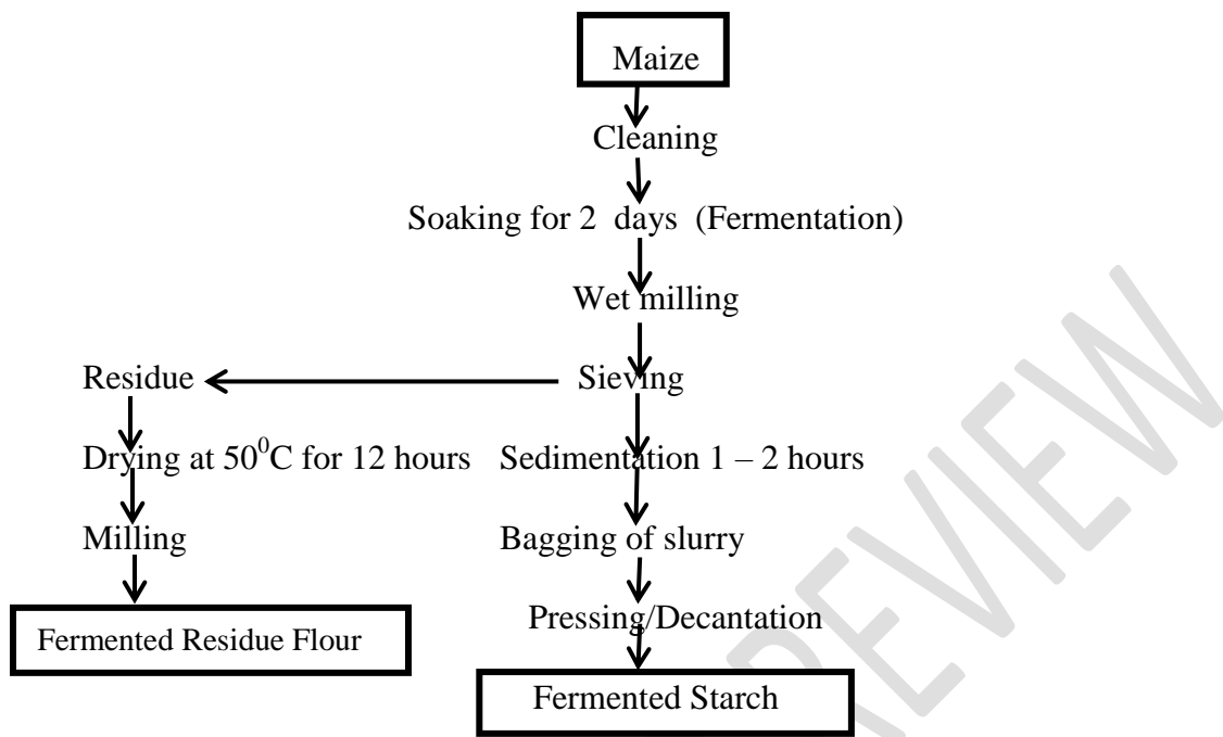
Fig. 1: Flow diagram for fermented maize residue
