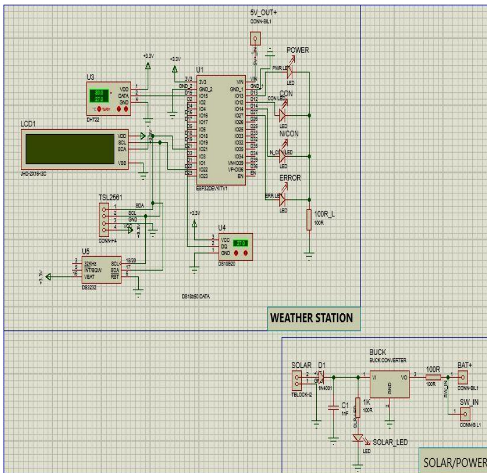
Fig. 6. Circuit diagram
