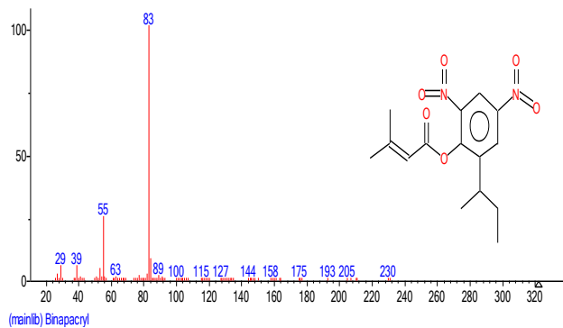
Fig. 2i. Mass spectrum of Binapacryl structure
