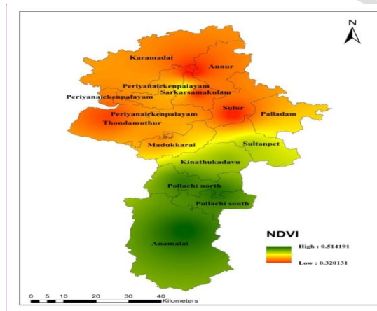
Fig 13: NDVI for AVHRR (1992-2015) composite data
