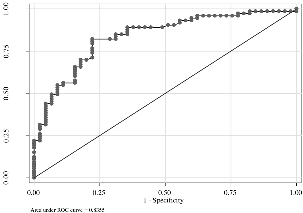
Fig. 2. ROC Curve
