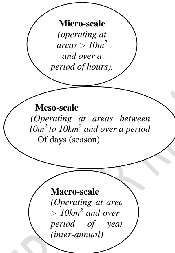
Fig.II: Combined spatio-temporal temperature changes scale (Guderson, et al. , 1995) In: Rivers Moore and Jewitt, 2004)
