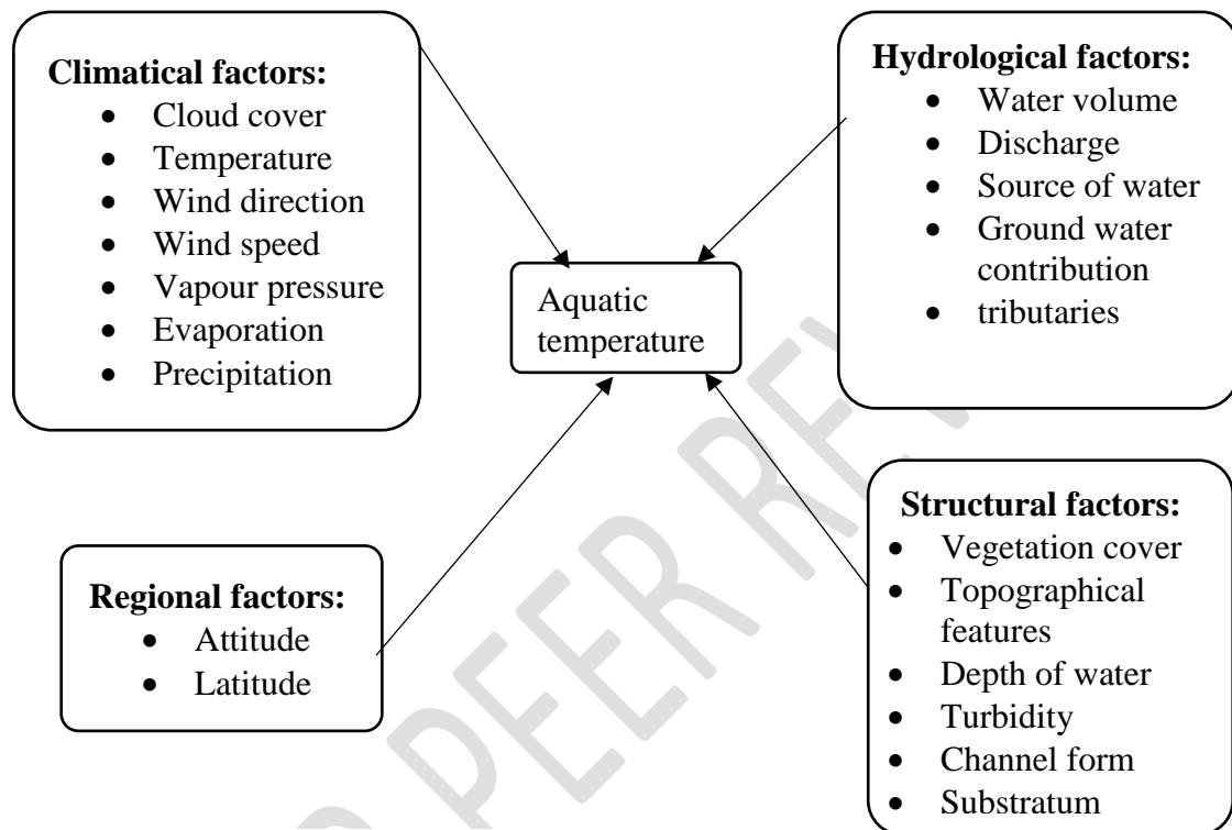
Fig. 1: Factors affecting aquatic temperature in ecological systems (Dallas, 2008).
