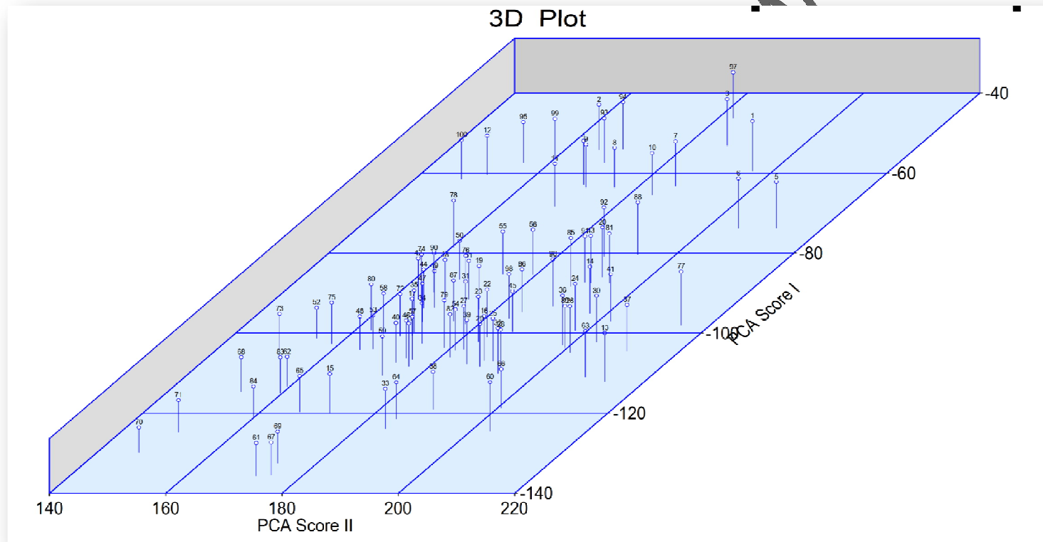
Fig.2. Three dimensional representational of PCA Biplot.
