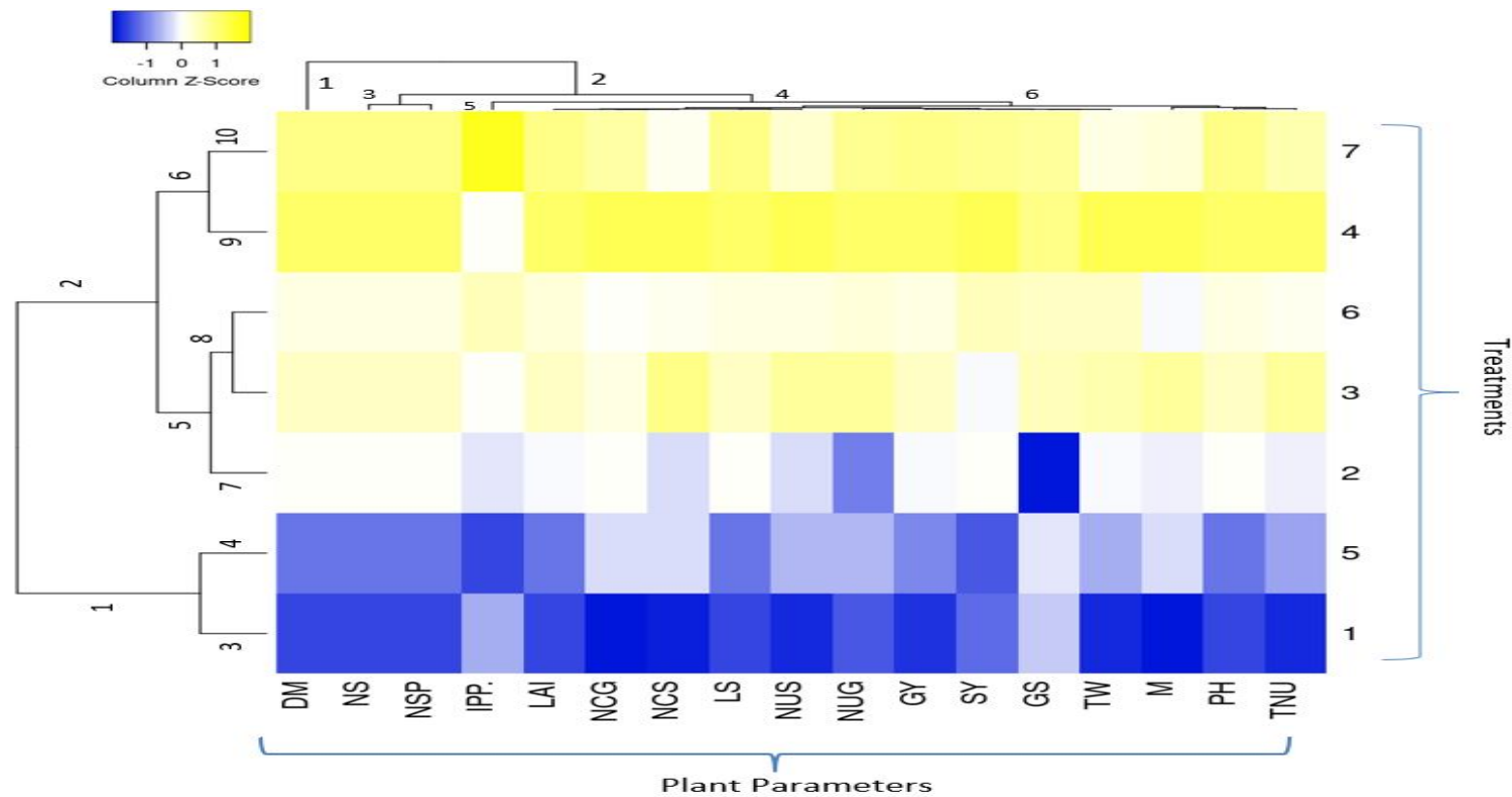
Fig. 2. Clustered heat map of the effect of different treatment combination on growth, yield and economic parameters of wheat; DM= Dry matter accumulation; NS= No. of shoots, NSP=No. of spike/m 2 ; IPP= Initial plant population; LAI= Leaf area index; NCG= Nitrogen content in grain; NCS= Nitrogen content in spike; LS= Length of spike; NUS= Nitrogen uptake in spike; NUG= Nitrogen uptake in grain; GY= Grain yield; SY= Straw yield; GS= Grain spike -1 ; TW= Test weight; M= Maturity; PH= Plant height; TNU= Total Nitrogen uptake.
