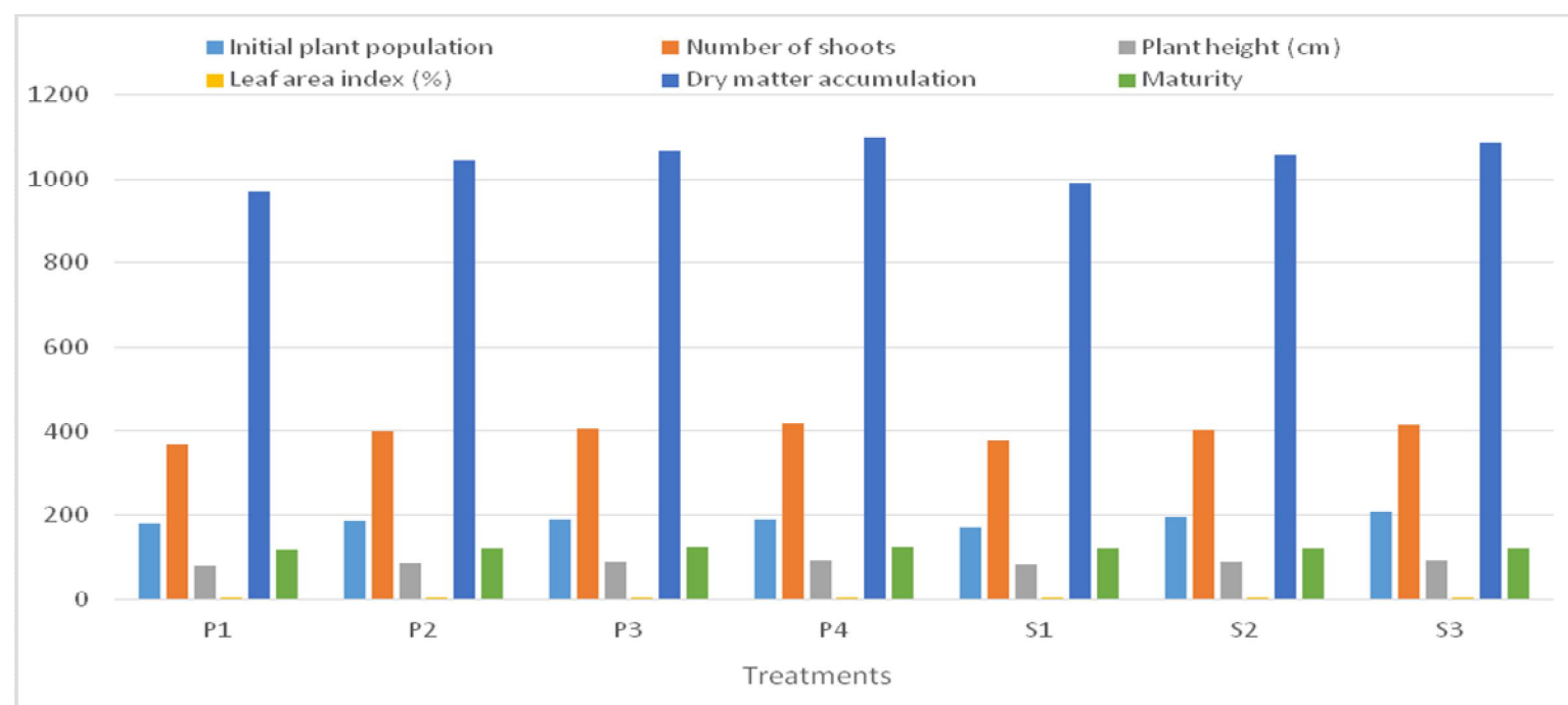
Fig. 1. Effect of different phosphorus levels and row spacing on growth parameters of wheat
