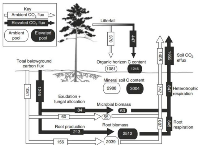
FIGURE 4. Underground carbon budgets for a warm-temperate forest exposed to elevated atmospheric CO2 at the Duke free-air CO2 enrichment (FACE) site. Ambient CO2 is shown in white, while elevated CO2 is shown in black. Ovals reflect pools and have units of g C m -2 ; squares within arrows reflect fluxes of C and have units of g C m -2 year -1 (Drake et al. 2011)
