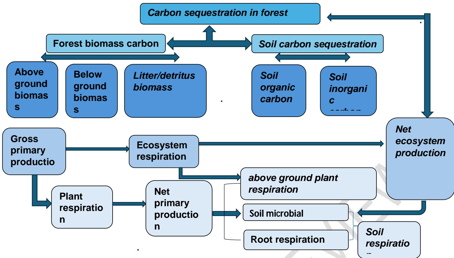
Figure 3. Carbon sequestration in forest ecosystems, including major carbon pools and fluxes (Hui et al. 2015)
