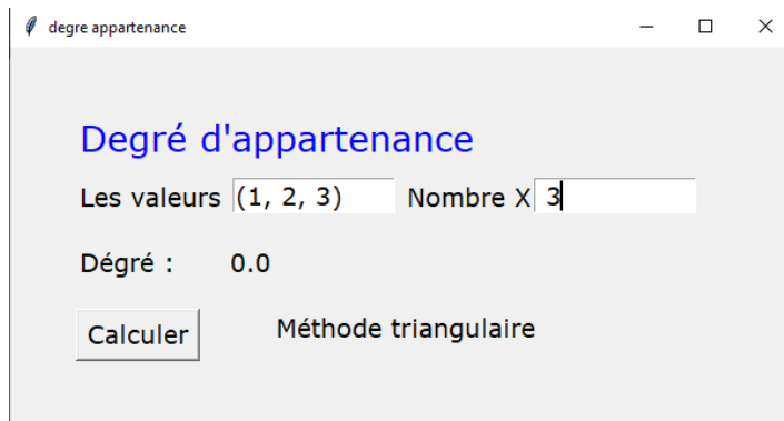
Figure 3: Calculation of Membership Degree Search ( Fuzzification ) 3
