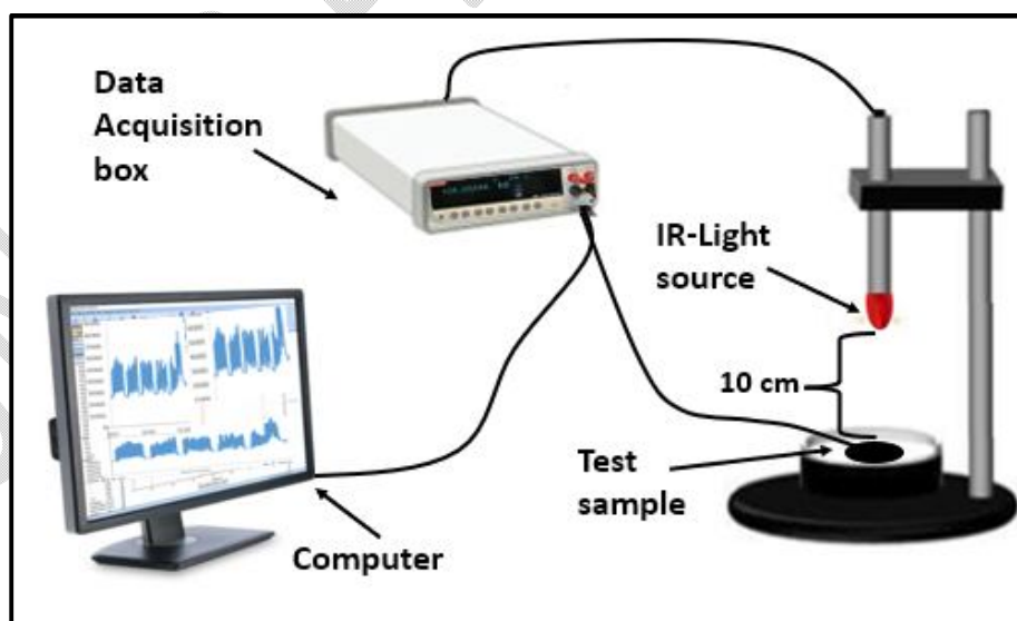
Fig. 2. The schematic representation of the data collection using the IR lamp.
