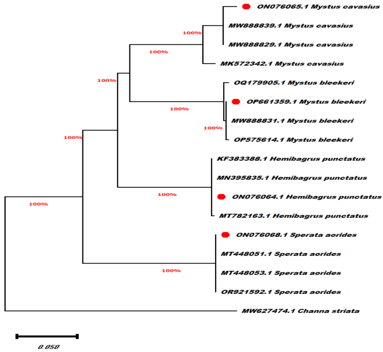
Fig.5. Phylogenetic analysis by using Neighbor-Joining method.
