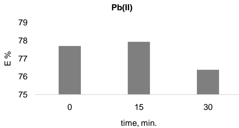
Fig. 9. Influence of time (minutes) on the removal efficiency of Pb(II) ions using sodium carbonate
