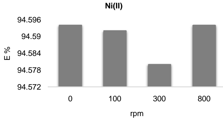
Fig. 2. Influence of solution mixing speed (rpm) on the removal efficiency of Ni(II) ions using sodium carbonate Conditions: Ni(II) 500 mg/L, pH 8, t = 5 minutes
