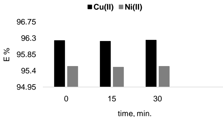
Fig. 11. Influence of time (minutes) on the removal efficiency of Cu(II) and Ni(II) ions in a binary multicomponent system using sodium carbonate
