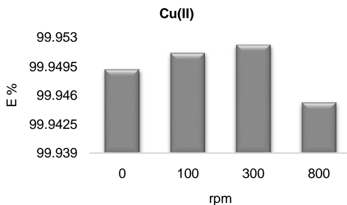
Fig. 1. Influence of solution mixing speed (rpm) on the removal efficiency of Cu(II) ions using sodium carbonate
