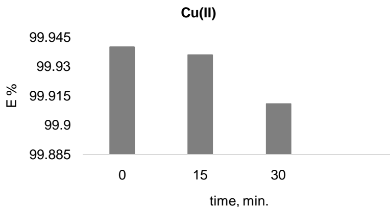
Fig. 7. Influence of time (minutes) on the removal efficiency of Cu(II) ions using sodium carbonate
