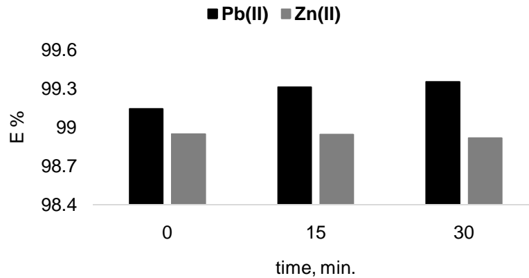
Fig. 12. Influence of time (minutes) on the removal efficiency of Pb(II) and Zn(II) ions in a binary multicomponent system using sodium carbonate Conditions: Pb(II) and Zn(II) 500 mg/L, pH 8, t = 5 minutes
