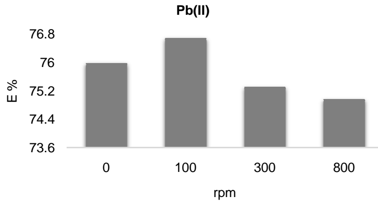
Fig. 3. Influence of solution mixing speed (rpm) on the removal efficiency of Pb(II) ions using sodium carbonate Conditions: Pb(II) 500 mg/L, pH 8, t = 5 minutes
