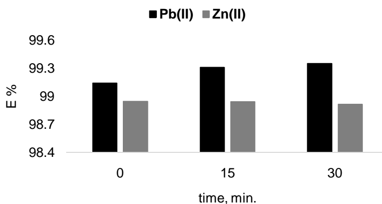
Fig. 12. Influence of time (minutes) on the efficiency of precipitation of Pb(II) and Zn(II) ions in a binary multicomponent system using sodium carbonate Conditions: Pb(II) and Zn(II) 500 mg/L, pH 8, t = 5 minutes
