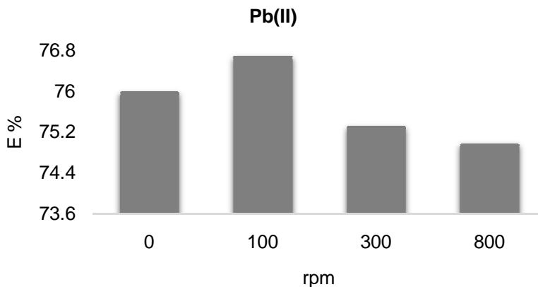
Fig. 3. Influence of solution mixing speed (rpm) on the efficiency of precipitation of Pb(II) ions using sodium carbonate Conditions: Pb(II) 500 mg/L, pH 8, t = 5 minutes
