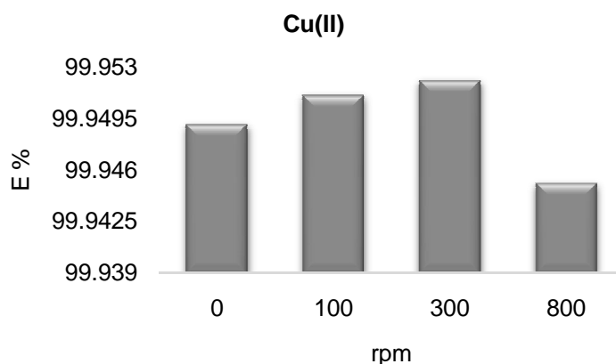
Fig. 1. Influence of solution mixing speed (rpm) on the efficiency of precipitation of Cu(II) ions using sodium carbonate
