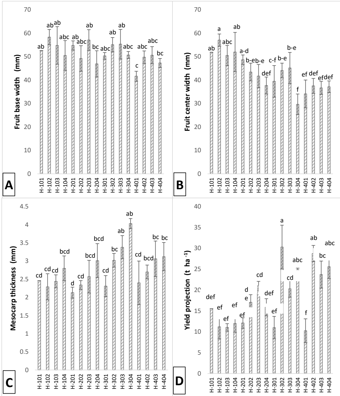
Figure 2. response of the experimental poblano chili bell pepper hybrids in fruit base width (a), fruit center width (b), mesocarp thickness (c) and yield projection (d), ANOVA p \leq 0.05 , Tukey's test of means ( p \leq 0.05 ), vertical bars correspond to standard deviation.
