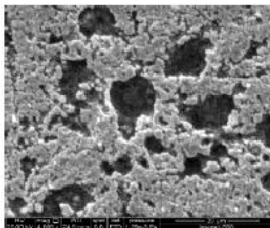
With Cu-complex
