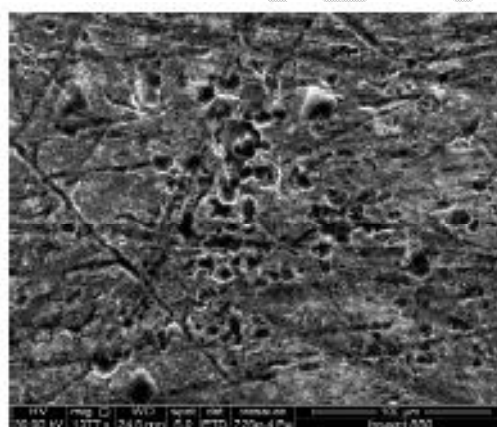
With Co-complex
